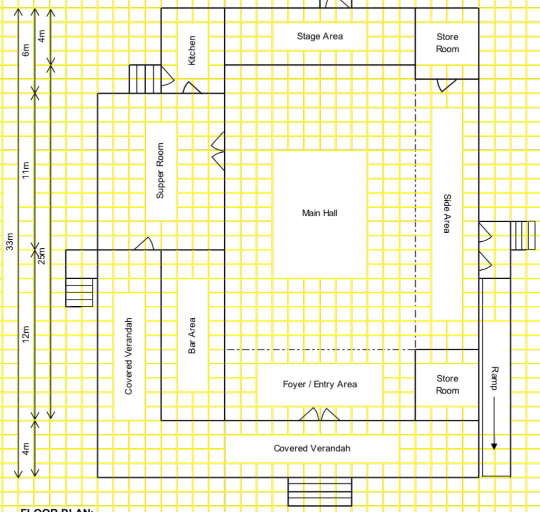
FLOOR PLAN:
